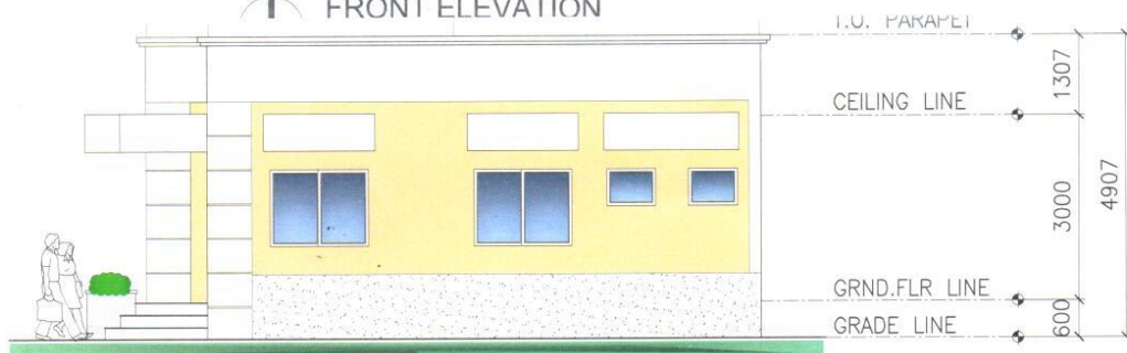
FRONT ELEVATION
