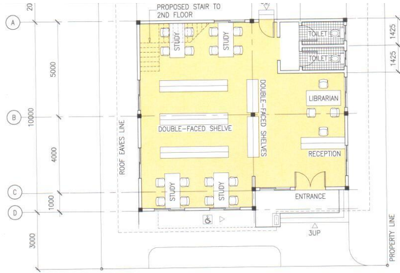
GROUND FLOOR PLAN SCALE : 1:100M
